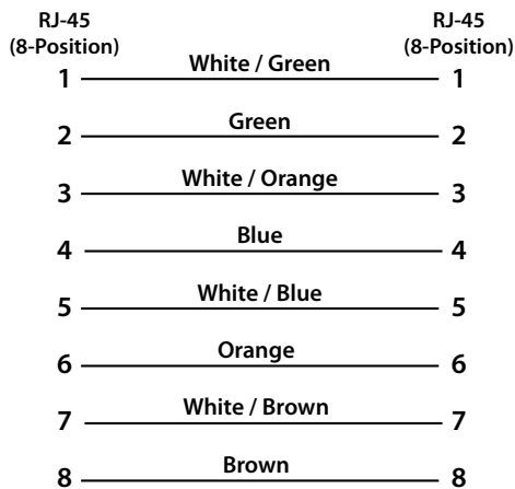
TIA/EIA 568A Straight-Through CAT5e or CAT6
