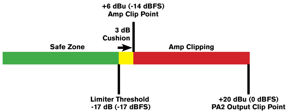
Gain Structure & Limiter Threshold Setting Example
