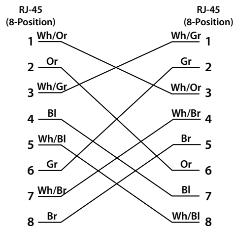
TIA/EIA 568B Crossover CAT5e or CAT6
