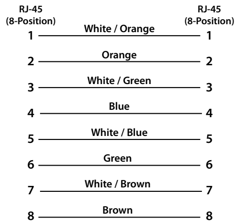
TIA/EIA 568B Straight-Through CAT5e or CAT6
