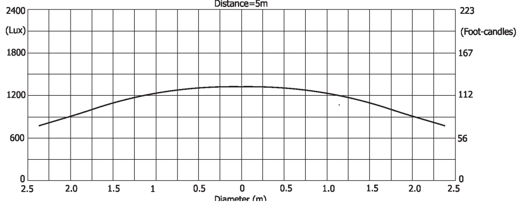
Illuminance distribution
