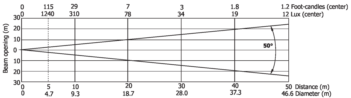
Illuminance distribution
