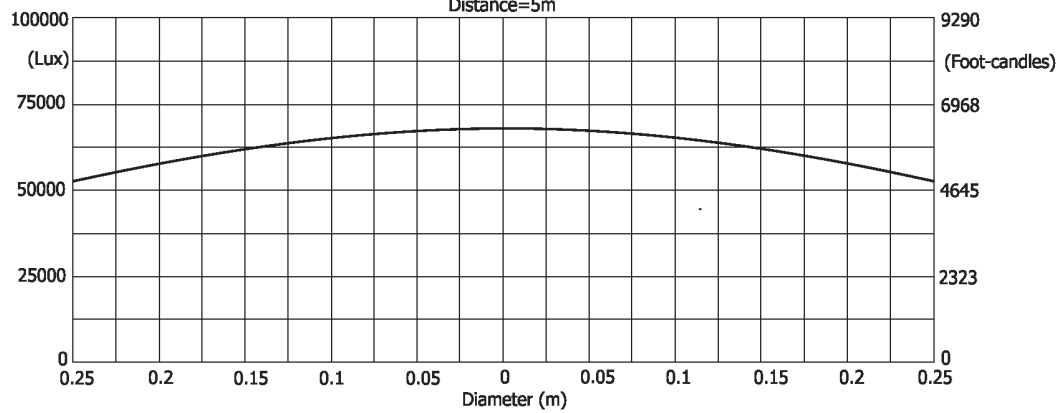
Illuminance distribution
