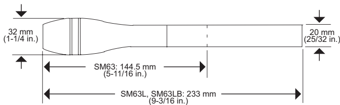
OVERALL DIMENSIONS
