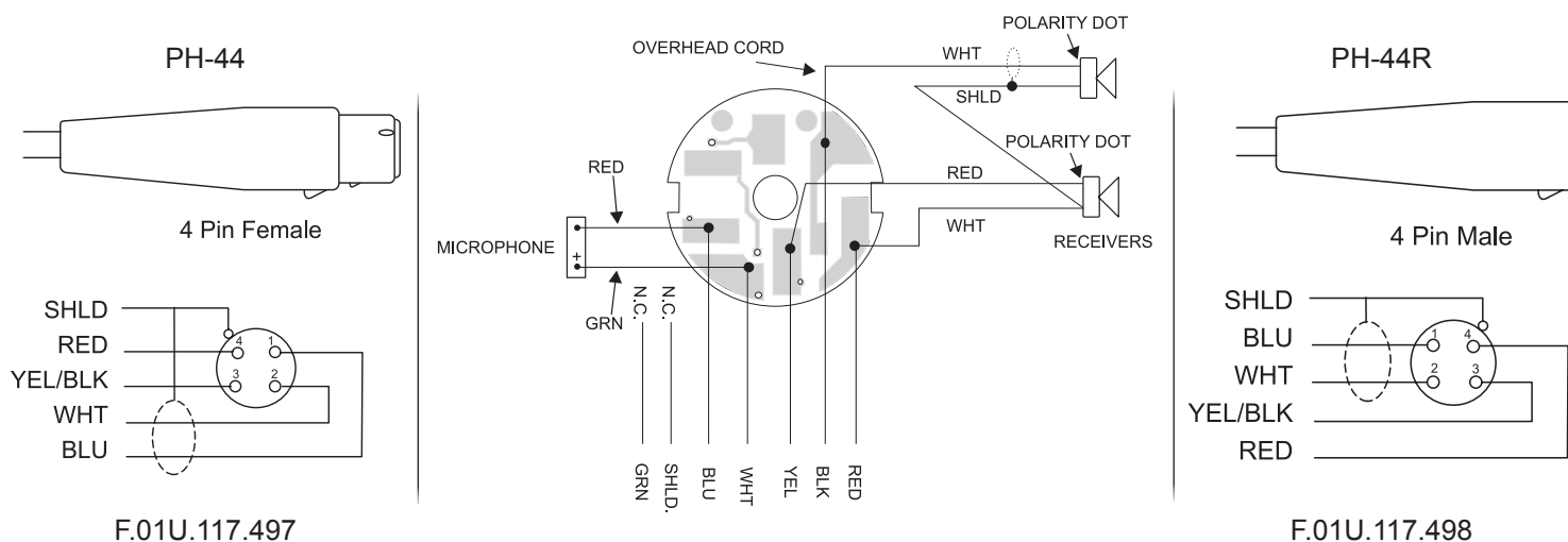
Wiring Diagram
